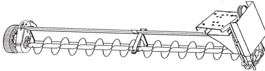
9" O.D. 1/4" Flight on 2 7/8" tube Drive includes 3 to 1 Oil Bath Reducer Capacity rated at ~1280 BPH per 100 RPM
