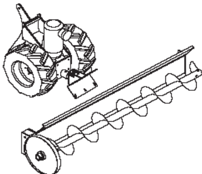
12" O.D. 1/4" Flight on 2 7/8" tube
